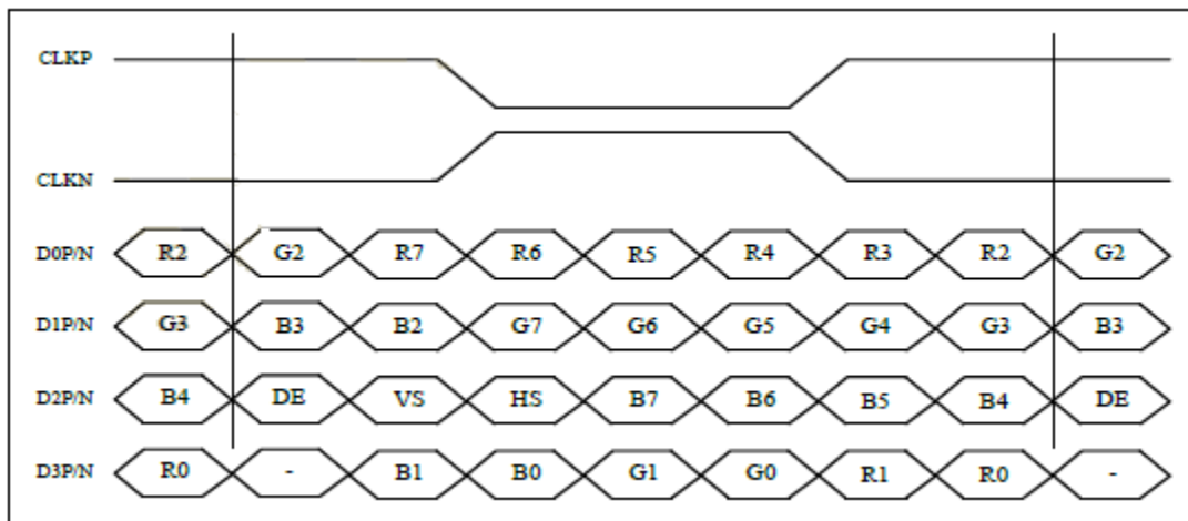
Figure 3: 8-bit LVDS JEIDA input timing
