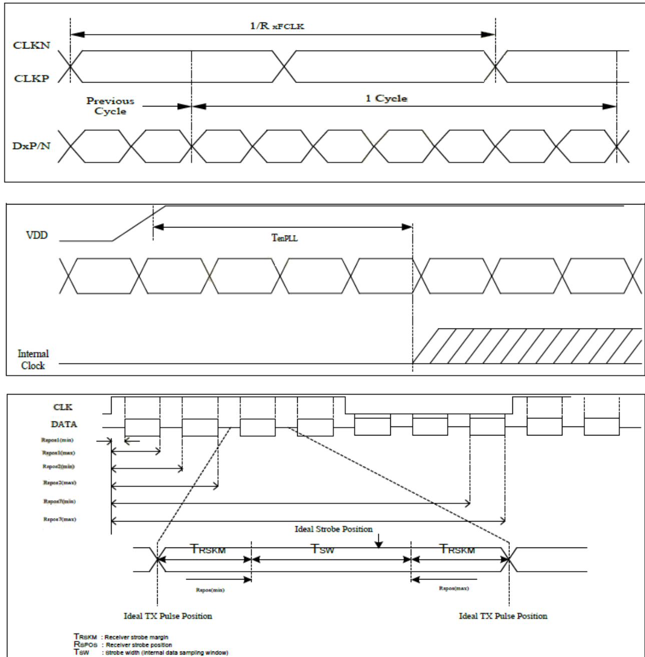
Figure 4: LVDS figure
