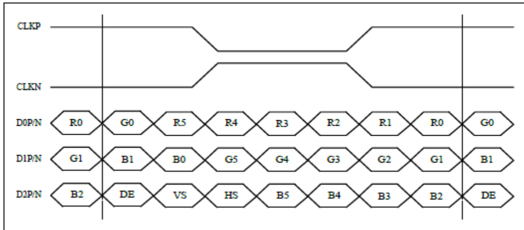
Figure 1: 6-bit LVDS input timing
